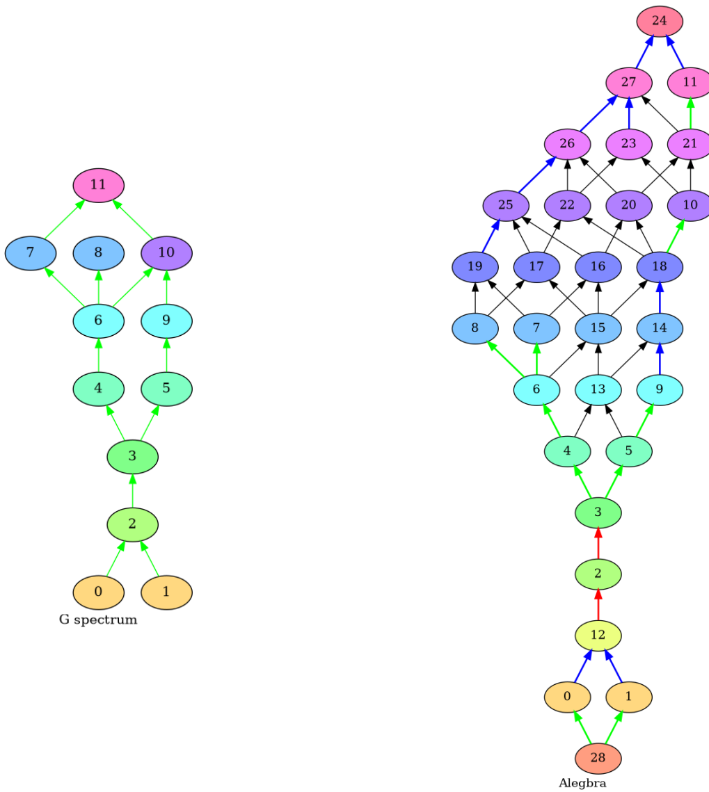
Fig. 5 A Heyting algebra and its spectrum
