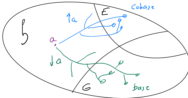
Fig. 1 Basis and co-basis
