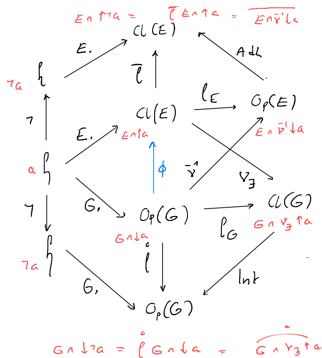
Fig. 3 Relations between topologies
