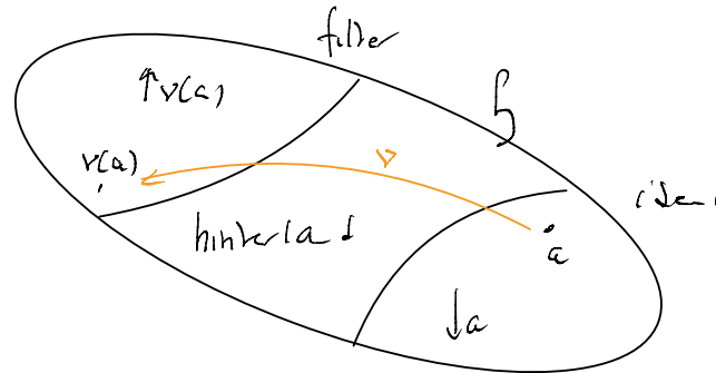
Fig. 2 Irrelevant operator
