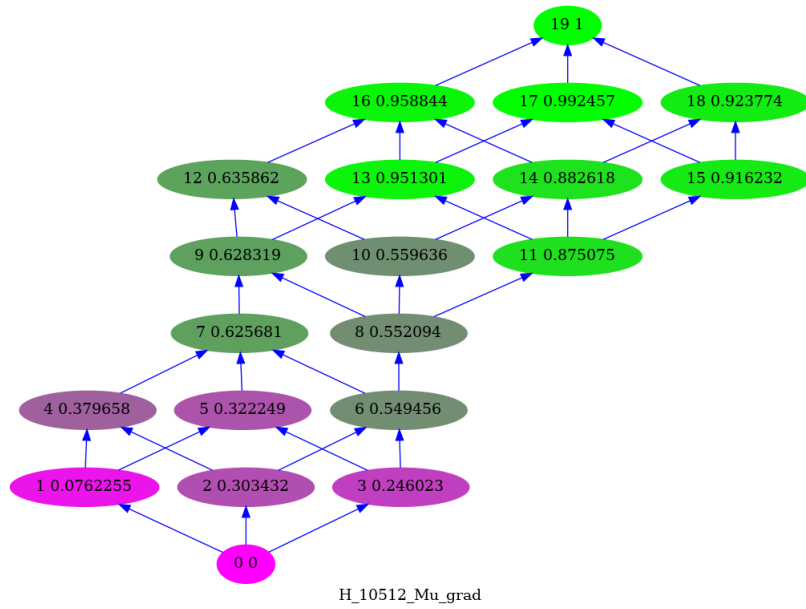
Figure 4: Probability. Incidentally, we can introduce a notion of information by -\log \mu . \top contains no information because \log \mu(\top) = \log 1 = 0 , while -\log \mu(\perp) = -\log 0 = \infty suggests that infinite information would be needed to demonstrate the absurd.
