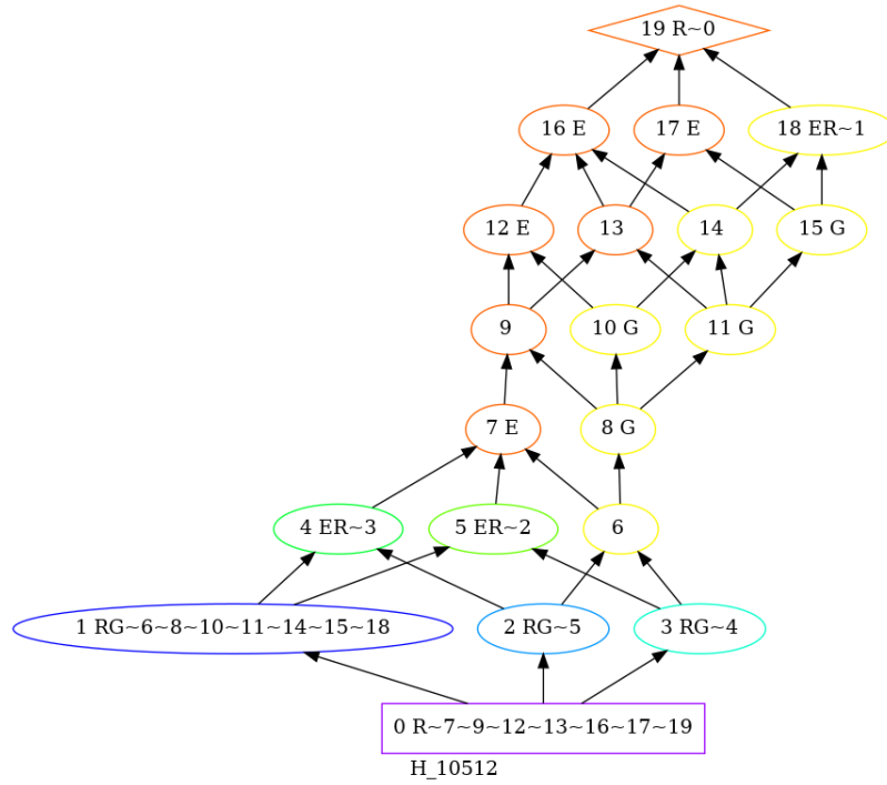
Figure 1: Hasse diagram of a Heyting algebra.
