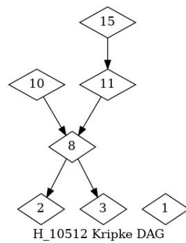
Figure 2: Order relationship restricted to primary filter infs.
