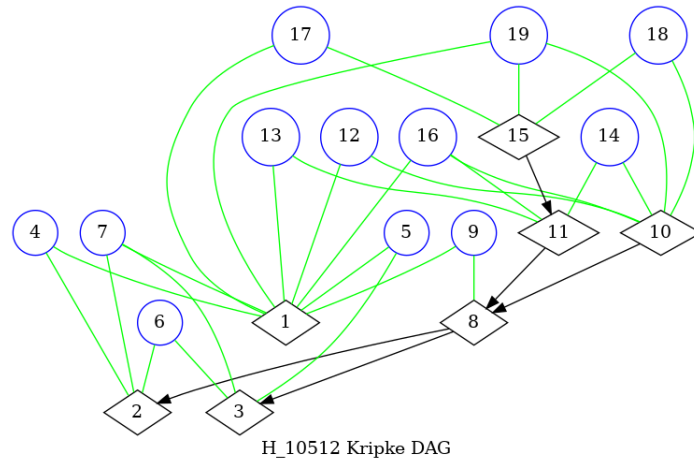
Figure 3: Extension of \mu_g by antichains. To obtain the prob of an element outside G , we sum the probs of the ends of its outgoing arrows.
