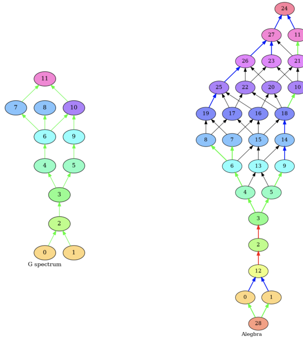
Figure 5: Heyting algebra and its spectrum
