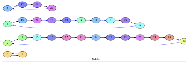
Figure 6: \nu -orbits
