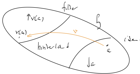
Figure 2: Irrelevant operator
