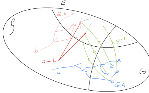
Figure 4: Implication
