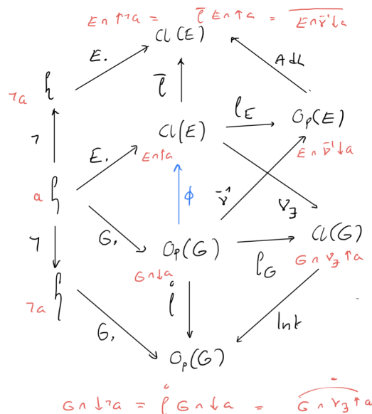
Figure 3: Relations between topologies
