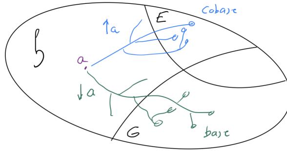
Figure 1: Basis and co-basis
