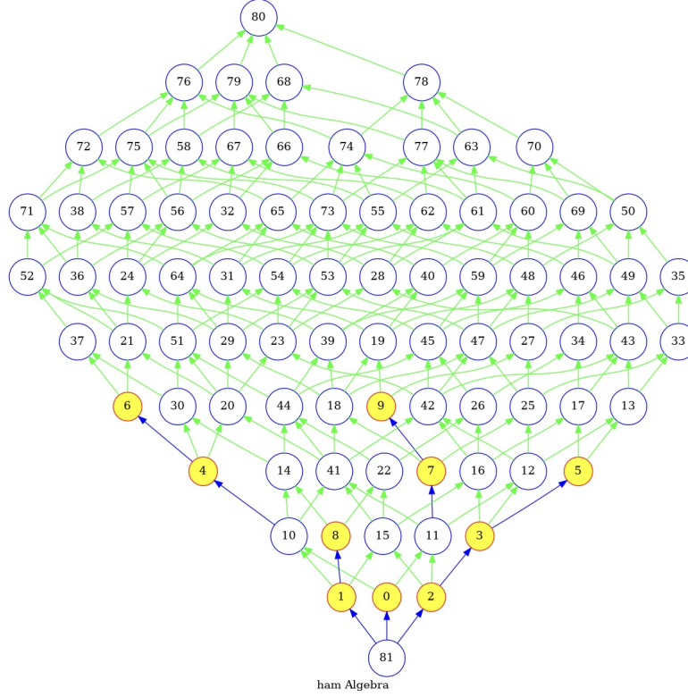
Figure 5: Hamiltonian algebra
